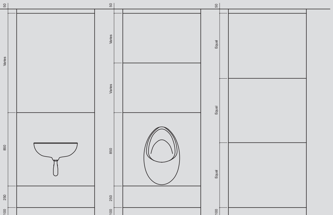
Floor to Ceiling 3 No. Panels
