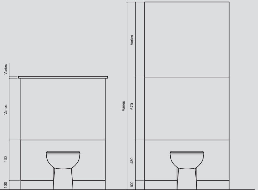
Half Height Duct & Access 2 No. Panels
